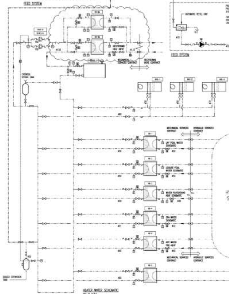
HEATER WATER SCHEMATIC REF TO SCALE
